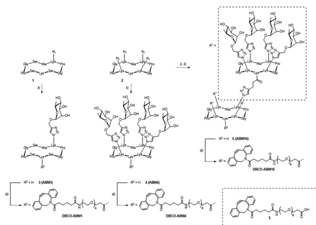
Scheme 2 Synthesis of DBCO-ABM conjugates. Reagents and conditions: i) pentynoic acid NHS ester, DIPEA, DMF, 2 h, r.t.; ii) propargyl \alpha -L-rhamnopyranoside 2 , CuSo_4 \cdot 5H_2O , THPTA, sodium ascorbate, DMF/PBS (p.H. 7.5) (1:1), 2h., r.t.; iii) 5 , PyBOP, DIPEA, DMF 4 h, r.t.
