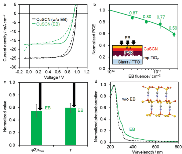
Fig. 2 (a) JV curve of the best-performing regular PSC of Device 4 (FTO/ c -TiO 2 /mpTiO 2 /PVK/CuSCN/Au) with (green curves) and without EB exposure (black curves, F_{EB} = 2.5 \times 10^{15} \text{ cm}^{-2} ). The solid and dashed lines are the reverse and forward scans, respectively. (b) Decrease in the PCE upon EB irradiation normalized by the initial PCE. Average values are superimposed. Schematic shows the device structure and EB irradiation geometry. (c) \phi\Sigma\mu_{\text{max}} of TRMC transients normalized by that of the as-prepared CuSCN layer ( \lambda_{\text{ex}} = 355 \text{ nm} , I_0 = 2.0 \times 10^{16} \text{ photons cm}^{-2} \text{ pulse}^{-1} ). The arrows represent the change from the original value without EB irradiation. (d) Normalized photoabsorption spectra of the CuSCN film before (black line) and after EB exposure (green line, F_{EB} = 2.5 \times 10^{15} \text{ cm}^{-2} ). The crystal structure of CuSCN (Materials Project, DOI: https://doi.org/10.17188/1270619 ) is superposed.
