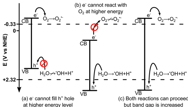
Fig. 6 Schematic illustration of redox potential for \cdot\text{OH} and \text{O}_2\cdot^- showing (a) a semiconductor with sufficiently negative CB to allow \text{O}_2 + \text{e}^- , but VB too negative to allow \text{H}_2\text{O} + \text{h}^+ as \text{H}_2\text{O} cannot donate an electron to fill the more negative hole in the VB of the semiconductor. (b) A semiconductor with sufficiently positive VB such that \text{H}_2\text{O} may donate an electron to fill the hole, however the CB is too positive meaning \text{O}_2 cannot accept \text{e}^- . (c) A semiconductor with both a sufficiently negative CB, and a sufficiently positive VB. This semiconductor would be capable of facilitating both reactions but has an increased band gap, limiting its solar spectrum adsorption range. Heterojunctions (Fig. 7) can be used to reduce this band gap whilst maintaining the redox potentials. Figure is for illustrative purposes only and is not drawn to scale.
