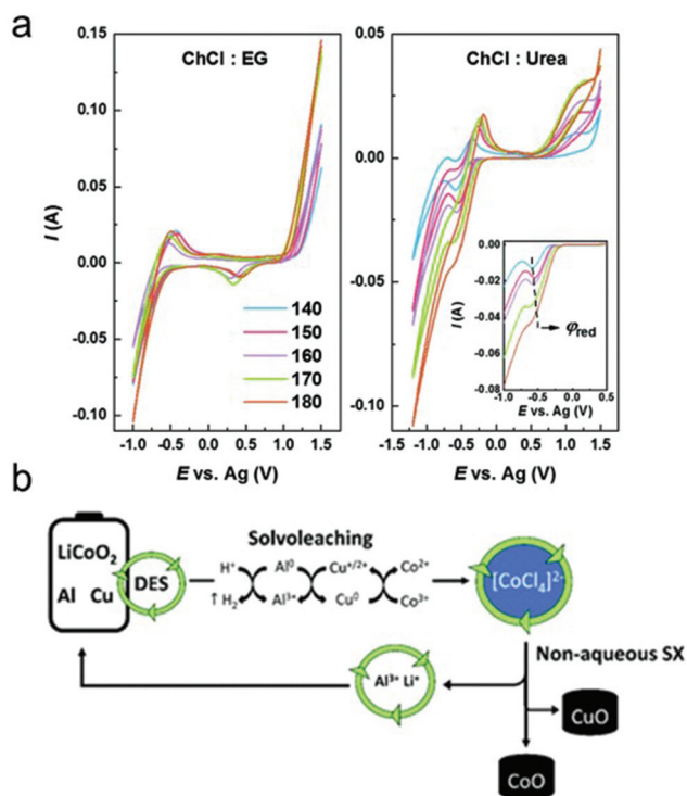
Fig. 6 The redox reactions in the DESs based metal recovery processes. (a) Cyclic voltammograms of \text{ChCl} : \text{ethylene glycol} (left) and \text{ChCl} : \text{urea} (right) DESs recorded at a fixed scan rate of 50 \text{ mV s}^{-1} . Reprint with permission from ref. 154, Copyright © 2020, Royal Society of Chemistry. (b) Schematic diagram of cobalt recovery from lithium-ion battery cathode materials using \text{ChCl} : \text{citric acid DES} with the acceleration of aluminum and copper metal. Reprint with permission from ref. 155, Copyright © 2020, Royal Society of Chemistry.
