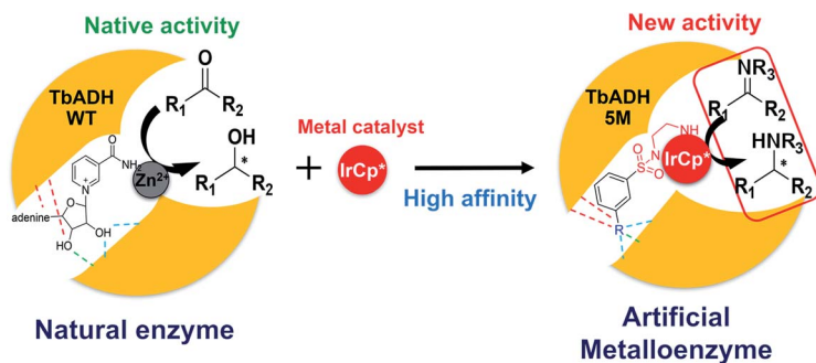
Fig. 1 Schematic representation of the design of ArMs: left, the natural catalysis in TbADH WT involving \text{NADP}^+ and a catalytic \text{Zn}^{2+} ; right, the supramolecular insertion of an iridium piano stool complex (red) inside the \text{NADP}^+ cofactor pocket and \text{Zn}^{2+} binding region of TbADH 5M with high affinity induced by the anchor substructure (R).
