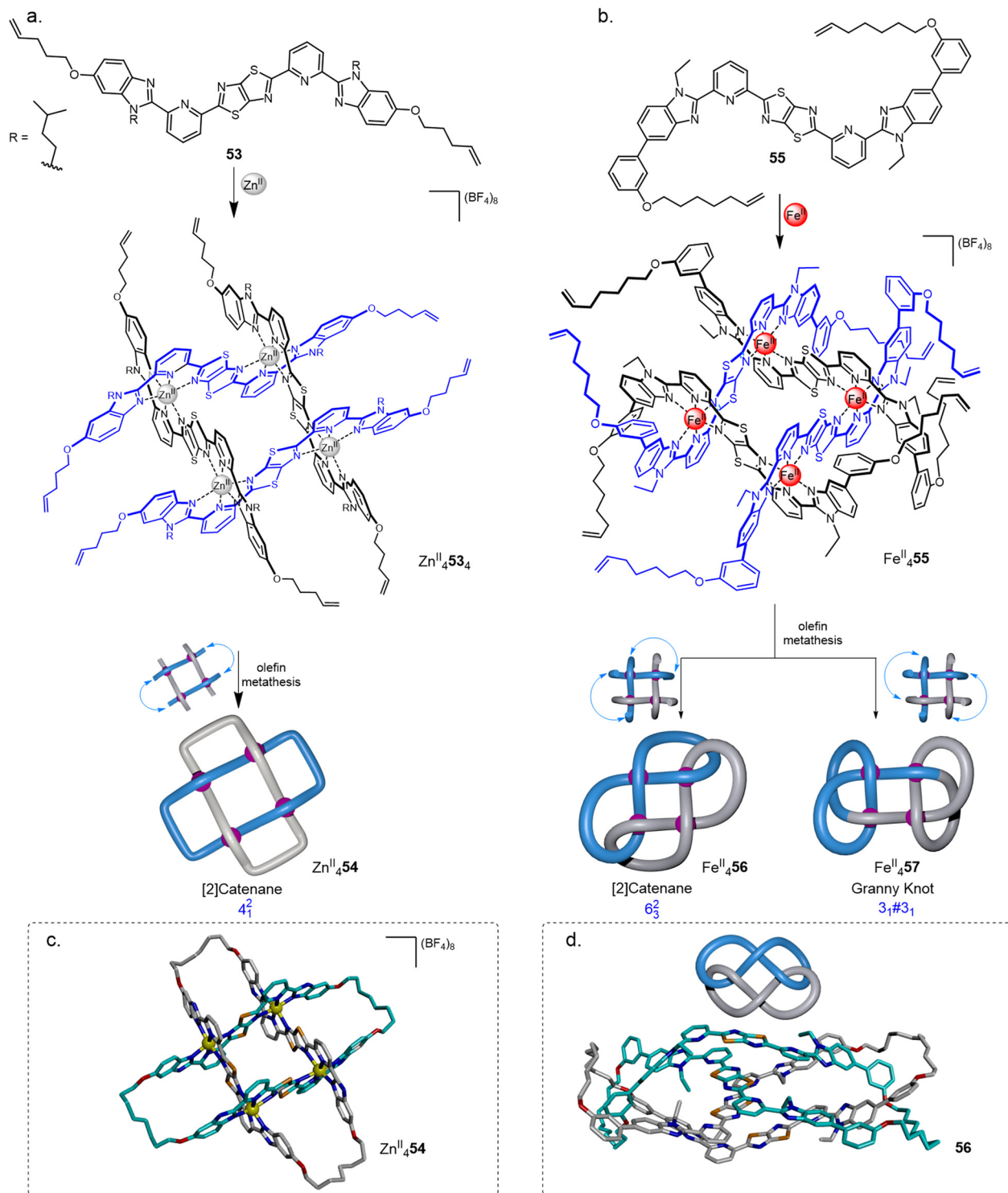
Fig. 20 Synthesis of 2 × 2 interwoven molecular grids and their closures by olefin metathesis to generate (a) Solomon link 54 , 14 or (b) 6 3 2 link 56 and granny knot 57 , 15 X-ray crystal structures of (c) Zn II 4 54 and (d) demetallated link 56 .
