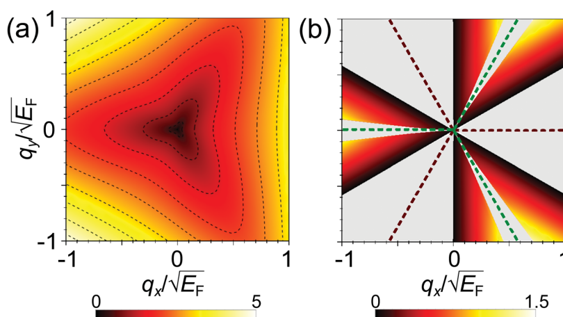
Fig. 2 Contour plots of the dispersion of (a) the 2D plasmon normalized energy \frac{\omega_{2DP}(\mathbf{q})}{E_F} and (b) the acoustic plasmon normalized energy \frac{\omega_{AP}(\mathbf{q})}{E_F} in the q_x - q_y plane, for a system with a free-electron-like dispersion with triangular anisotropy. The black dashed lines in (a) highlight curves of constant energy \omega_{2DP} . Brown and green dashed lines in (b) indicate the symmetry directions of the band structure with the lowest and the largest effective masses, respectively. The gray regions represent the momentum \mathbf{q} regions where the acoustic plasmon does not exist.
