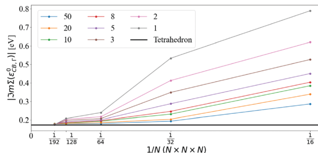
Fig. 3 Convergence of \Im m\Sigma_{\text{CBM}}(\epsilon_{\text{CBM}}^0) using the DM approach with N for different values of \eta = 50, 20, 10, 8, 5, 3, 2 , and 1 meV (indicated in the legend) at 300 K. The black line denotes the reference value obtained with the tetrahedron method and N = 160 .
