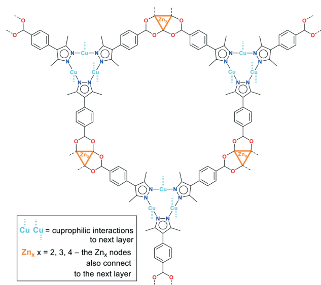
Scheme 2 Common features of the structures of 1–3 with \text{Zn}_x nodes of different nuclearities ( x = 2\text{--}4 ) and the trigonal \{\text{Cu}_3(\text{mpba})_3\}^{3-} nodes giving a hexagonal-ring layer. Both the \text{Zn}_x nodes and the cuprophilic interactions from \{\text{Cu}_3(\text{mpba})_3\}^{3-} connect to the next layer.
