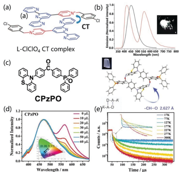
Fig. 13 (a) Structure of L\text{-Cl}\cdot\text{ClO}_4 and the presentation of the formation of a CT complex. (b) Fluorescence spectra of L\text{-Cl}\cdot\text{ClO}_4 in dilute EtOH solution ( 10^{-5} M) (black line) and the crystalline state (red line) (excited at 290 nm). Photographs of L\text{-Cl}\cdot\text{ClO}_4 crystals were taken under 365 nm UV light. Reprinted with permission from ref. 94. Copyright 2014 The Royal Society of Chemistry. (c) The chemical structures, single-crystal structures, and luminescence pictures of CPzPO. (d) Changes in the emission spectra and CIE coordinates of CPzPO by gradual addition of methanol in benzene solution. (e) Temperature-dependent emission decay spectra of CPzPO at 564 nm in the crystalline state. Reprinted with permission from ref. 95. Copyright © 2017 Wiley-VCH Verlag GmbH & Co. KGaA, Weinheim.
