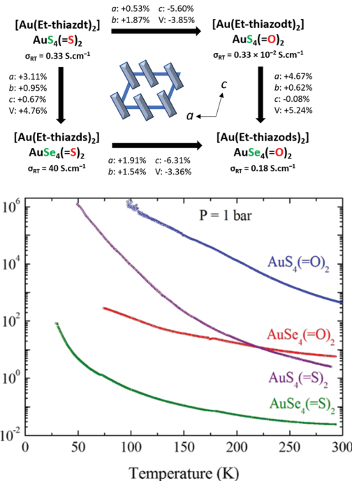
Fig. 13 Top: Evolution of the unit cell parameters within the series. Bottom: Temperature dependence of the resistivity of the four complexes at ambient pressure measured in single crystals. Adapted with permission from Yzambart, G., Bellec, N., Nasser, G., Jeannin, O., Roisnel, T., Fourmigué, M., Auban-Senzier, P., Íñiguez, J., Canadell, E., & Lorcy, D. (2012). Anisotropic Chemical Pressure Effects in Single-Component Molecular Metals Based on Radical Dithiolenes and Diselenolene Gold Complexes. J. Am. Chem. Soc. , 134(41), 17138–17148. DOI: 10.1021/ja3065649. Copyright 2012 American Chemical Society.
