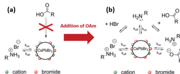
Fig. 13 Schematic representations of the dynamic surface stabilization of CsPbBr 3 NCs purified by acetone and dispersed in hexane (a) by oleylammonium bromide before the addition of excess OAm and (b) by oleylammonium bromide, oleylammonium oleate and OAm after the addition of excess OAm. The figure is modified with permission from ref. 33.
