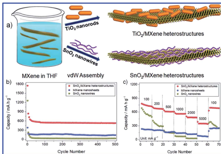
Fig. 30 (a) Scheme showing the self-assembly on MXene nanosheets, (b) their specific capacities at a current density of 1000 \text{ mA g}^{-1} and (c) rate capabilities for 70 cycles, 347 presented with permission and copyright.
