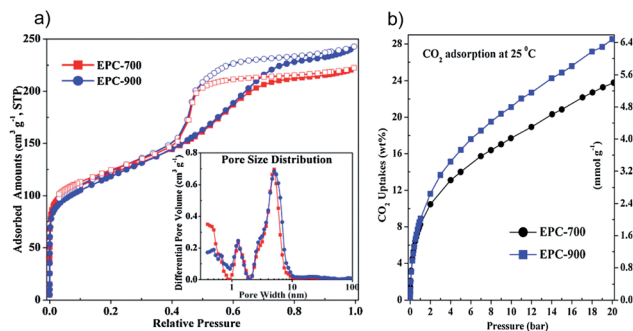
Fig. 18 (a) \text{N}_2 sorption isotherm (the pore size distribution is shown in the inset). (b) \text{CO}_2 adsorption isotherm at 25 \text{ }^\circ\text{C} . Reproduced with permission from ref. 174, copyright (2016) Elsevier.
