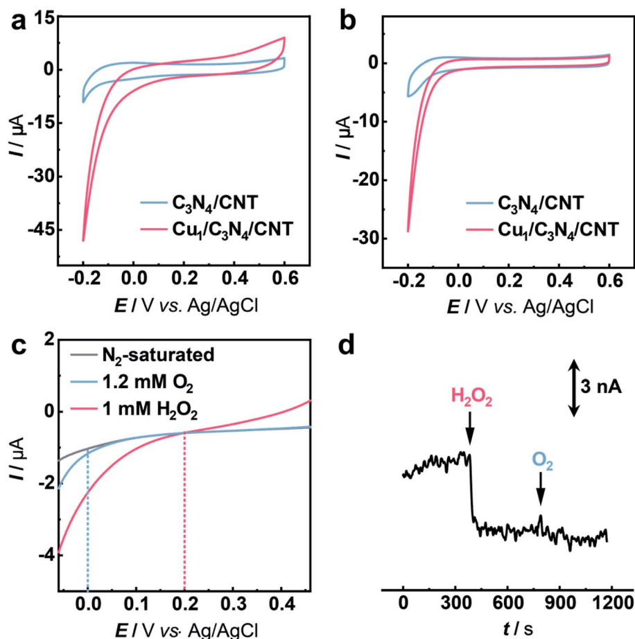
Fig. 3 Electrochemical study of the HPOR over the ORR. (a and b) CVs obtained with glassy carbon (GC) electrodes modified with C 3 N 4 /CNT (blue curve) and Cu 1 /C 3 N 4 /CNT (red curve) in aCSF (pH 7.4) in the presence of 5 mM H 2 O 2 (a) or under an O 2 atmosphere (ca. 1.2 mM O 2 ) (b). Scan rate: 50 mV s -1 . (c) LSVs obtained with the CuSAC-based electrode in aCSF without (gray curve) and with 1.2 mM O 2 (blue curve) or 1 mM H 2 O 2 (red curve) in aCSF under a N 2 atmosphere. Scan rate: 50 mV s -1 . (d) Amperometric response recorded at the SAC-based electrode with the addition of 5 \mu M H 2 O 2 and 50 \mu M O 2 in aCSF. Applied potential: 0.0 V vs. Ag/AgCl.
