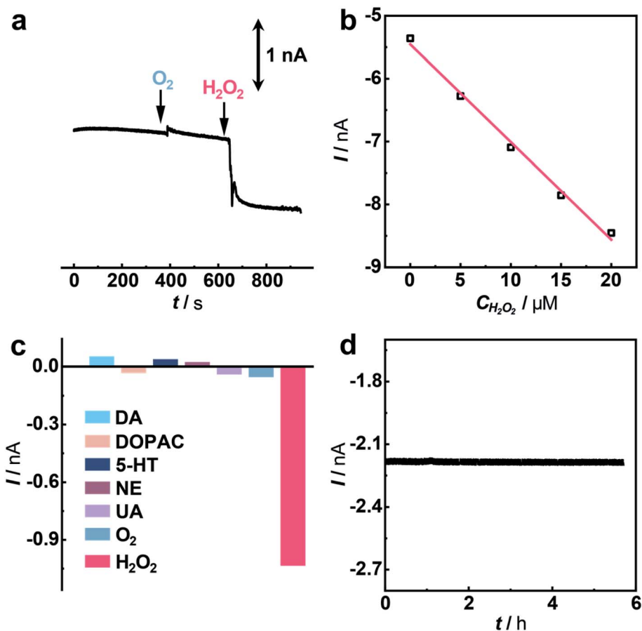
Fig. 5 Selective sensing of H_2O_2 with the CuSAC-based microsensors. (a) Amperometric responses recorded with the microsensors in aCSF toward the addition of 50 \mu M O_2 and 5 \mu M H_2O_2 . Applied potential: 0.0 V vs. Ag/AgCl. (b) Calibration curve for amperometric H_2O_2 detection obtained at the microsensors in aCSF toward successive addition of 5 \mu M H_2O_2 . Applied potential: 0.0 V vs. Ag/AgCl. (c) Amperometric responses recorded with the microsensors in aCSF toward 10 \mu M DA, 10 \mu M DOPAC, 10 \mu M 5-HT, 10 \mu M NE, 10 \mu M UA, 50 \mu M O_2 or 5 \mu M H_2O_2 . Applied potential: 0.0 V vs. Ag/AgCl. (d) Long-time amperometric i-t curve recorded with the microsensors in aCSF toward 5 \mu M H_2O_2 . Applied potential: 0.0 V vs. Ag/AgCl.
