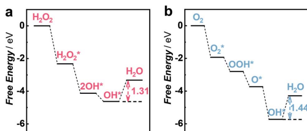
Fig. 4 DFT calculations for the HPOR and ORR on the Cu 1 /C 3 N 4 SAC. (a and b) Free energy diagrams of the HPOR (a) and ORR (b) at pH 7.0 on the active site of the Cu 1 /C 3 N 4 SAC.
