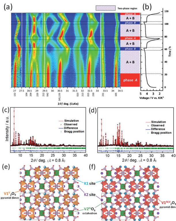
Fig. 7 (a) Contour map of operando XRD patterns in selected 2\theta regions and identified phase regions. (b) Charge–discharge profiles during the operando XRD measurement. Ex situ synchrotron XRD patterns of the KVPP electrodes (c) charged to 4.5 V and (d) discharged to 2.0 V. (e and f) Refined crystal structures by Rietveld method for the XRD patterns shown in panel ‘c’ and ‘d’, respectively.
