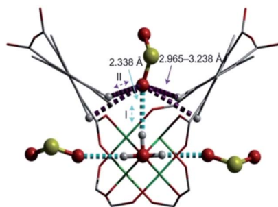
Fig. 2 Preferred binding sites for SO 2 molecules inside MFM-300(Al) determined by in situ PXRD. (I) Moderated hydrogen bond. (II) Weak hydrogen bond. Reprinted (adapted) with permission from ref. 37a. Copyright (2012) Springer Nature.
