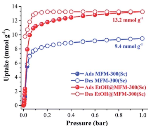
Fig. 4 SO 2 adsorption isotherm of scandium-based MFM-300 (blue isotherm) and after confinement of 2.8% EtOH (red isotherm). Reprinted with permission from ref. 37c. Published (2019) by The Royal Society of Chemistry.
