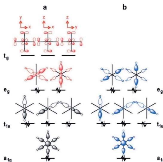
Fig. 5 Schematic MO diagrams for an O h -symmetric 12e - complex with d orbitals (a, red) and the MO diagram without d orbitals in 7c-12e - pattern of MO (b, blue). Reprinted (adapted) with permission from ref. 40c. Copyright (2015) John Wiley & Sons.
