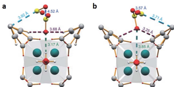
Fig. 3 Binding sites for SO 2 molecules within MFM-300(In) determined by single-crystal X-ray diffraction (a), and DFT calculations (b). Reprinted (adapted) with permission from ref. 37b. Copyright (2016) John Wiley & Sons.
