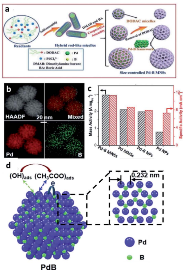
Fig. 8 (a) A scheme for the formation of Pd-intB MNSs. (b) EDX elemental mapping; Pd (red), B (green). (c) Mass and specific activities of Pd-intB MNSs, Pd MNSs, Pd-intB NPs and commercial Pd NPs collected in 1.0 M KOH and 1.0 M ethanol. This figure has been reproduced from ref. 77 with permission from Royal Society of Chemistry, copyright 2019. (d) A illustration of electrocatalytic EOR on the surfaces of Pd-intB. The inset shows the crystal structure of Pd-intB: Pd (purple), B (green). This figure has been reproduced from ref. 78 with permission from American Chemical Society, copyright 2020.
