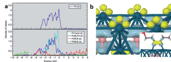
Fig. 9 DFT study of Pd-intB system. (a) DOS of pure Pd (top) and Pd-intB (bottom). (b) Electron-density difference isosurfaces show local electron-rich (light blue) and electron-poor regions (yellow) of Pd atoms (blue) with intB atoms (pink) due to states-mixing. Inset shows isolated HOMO/LUMO overlap of the adsorbate/surface interaction. This figure has been reproduced from ref. 37 with permission from Nature, copyright 2014.
