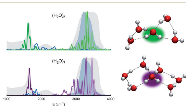
Fig. 3 Power spectra of the tetrahedrally coordinated monomer in different water clusters. Top left column: pentamer; bottom left column: heptamer. The combined excitation of the bending with the most coupled libration mode is also reported in dark blue. The liquid water IR spectrum is shown as shaded gray areas, and the MCR-Raman band (from ref. 12) for the stretches of tetrahedrally coordinated monomers in liquid water (light blue) is also presented.
