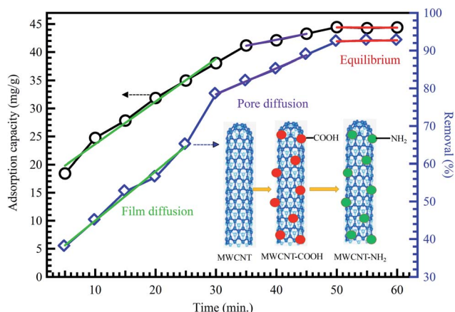
Fig. 10 Adsorption of methyl orange on MWCNTs, adapted with permission from ref. 41, copyright, Springer, 2019.
