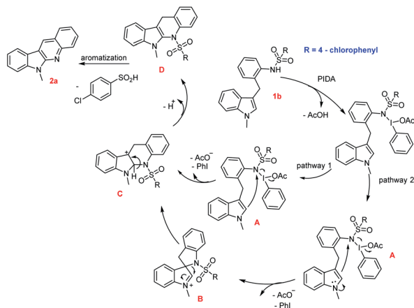
Scheme 2 Proposed mechanism.
