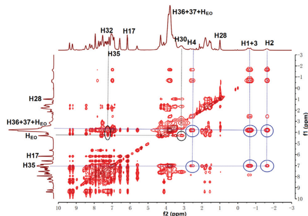
Fig. 2 NOESY NMR (400 MHz, \text{CDCl}_3 - \text{CD}_3\text{COCD}_3 = 3/1, v/v, 298 K) spectrum of M1 + M2 + M3 + M4 + Zn(OTf) _2 .
