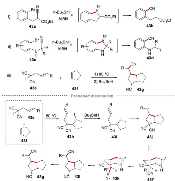
Scheme 43 Remote cyano migration to access nitriles.
