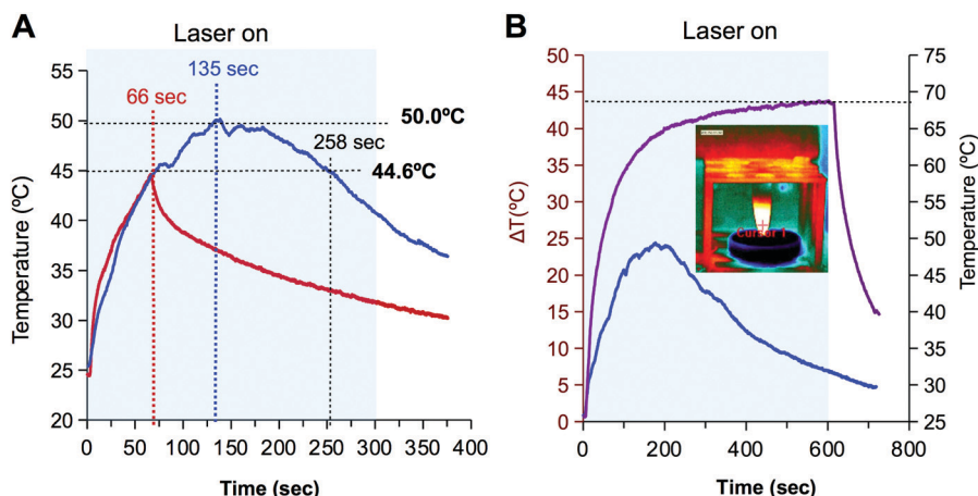
Fig. 5 Temperature increase as a function of time of 200 \mu L of a water solutions containing 133 \mu M IR783 (red), 72 \mu M LCD-2Na@IR780 (blue) and 285 \mu M LCD-2Na@IR780 (magenta) irradiated with a 808 nm NIR laser at a power of 1.2 \text{ W cm}^{-2} for 5 min (A) or 10 min (B). Inset B: Thermal image of the eppendorf containing the LCD-2Na@IR780 solution and the sample holder during the illumination. The temperature was recorded in real time with a high-resolution infrared camera.
