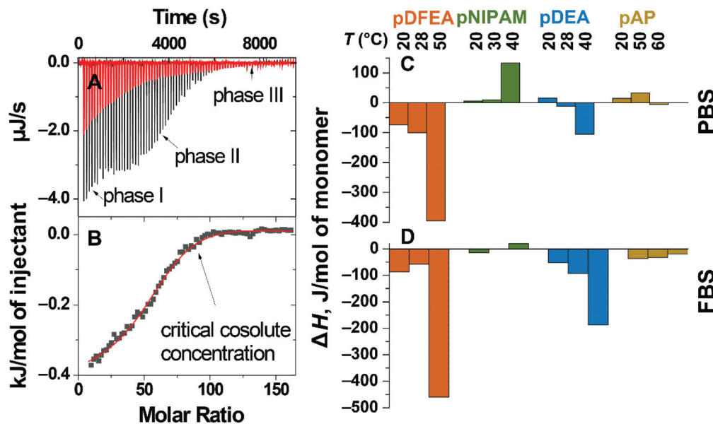
Fig. 5 ITC of 10.0 \text{ mg mL}^{-1} F3 (pDFEA solution in ultrapure water with PBS: heat flux as a function of time, titration of PBS to water (blank, red line), titration of PBS to polymer (black line) (A); integrated heat, normalised to 1 mol of F3 injectant (scatter), fit to model (line) (B). Enthalpies of the titration of 10.0 \text{ mg mL}^{-1} polymer solutions with PBS (C) and FBS (D), normalised to 1 mol of monomer units at three different temperatures. The values of enthalpies are outlined in Table S7.†
