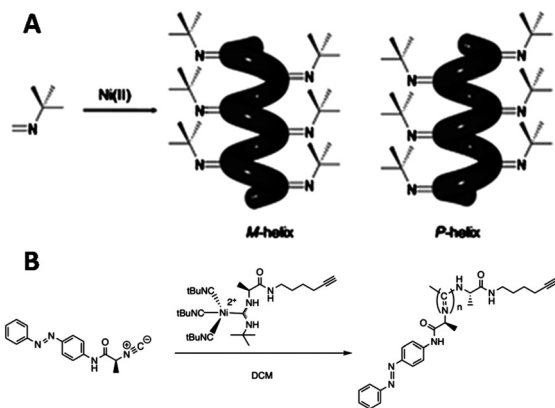
Fig. 31 A. Formation of stable helix by polymerizing tert -butyliisocyanide with a nickel(II) catalyst. Reproduced from ref. 214 with permission from the Royal Society of Chemistry, copyright (2011). B. Isocyanide polymerization with an alkyne-modified nickel(II) catalyst to introduce an alkyne handle on the polymer chain-end. Reprinted from ref. 225 with permission from John Wiley and Sons, copyright (1969).
