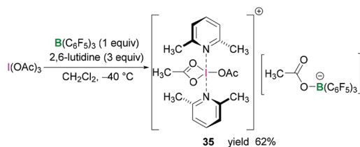
Scheme 14 Synthesis of diacetoxy iodonium 35 from \text{I(OAc)}_3 and \text{B(C}_6\text{F}_5)_3 .
