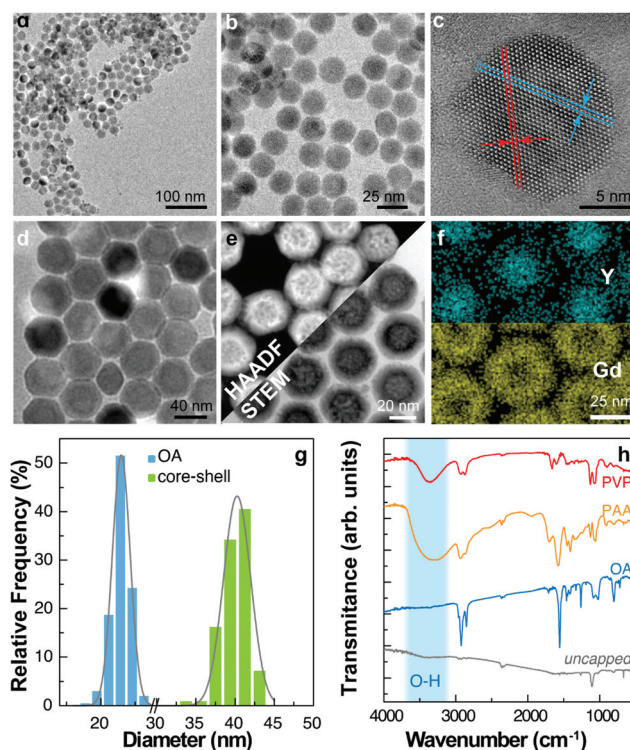
Fig. 1 Structure and (a and b) transmission electron microscopy images of the as-synthesized UCNP-OA. (c) High-resolution TEM image of a single UCNP. The plane separation d = 0.504 \pm 0.004 nm corresponds to the (100) plane of \beta\text{-NaYF}_4 . (d) TEM and (e) combined STEM and HAADF micrographs of core-shell nanoparticles. (f) Compositional mapping by EDS showing the yttrium and gadolinium profiles corresponding to the core and shell materials, respectively. (g) Size distribution extracted from the TEM images. The solid line corresponds to the best fit to a Gaussian distribution of mean \pm SD 21.5 \pm 1.5 nm (OA) and 40 \pm 4 nm (core-shell) ( r^2 > 0.97 ). (h) FTIR transmittance spectra of the uncapped UCNP and UCNP with different capping ligands.
