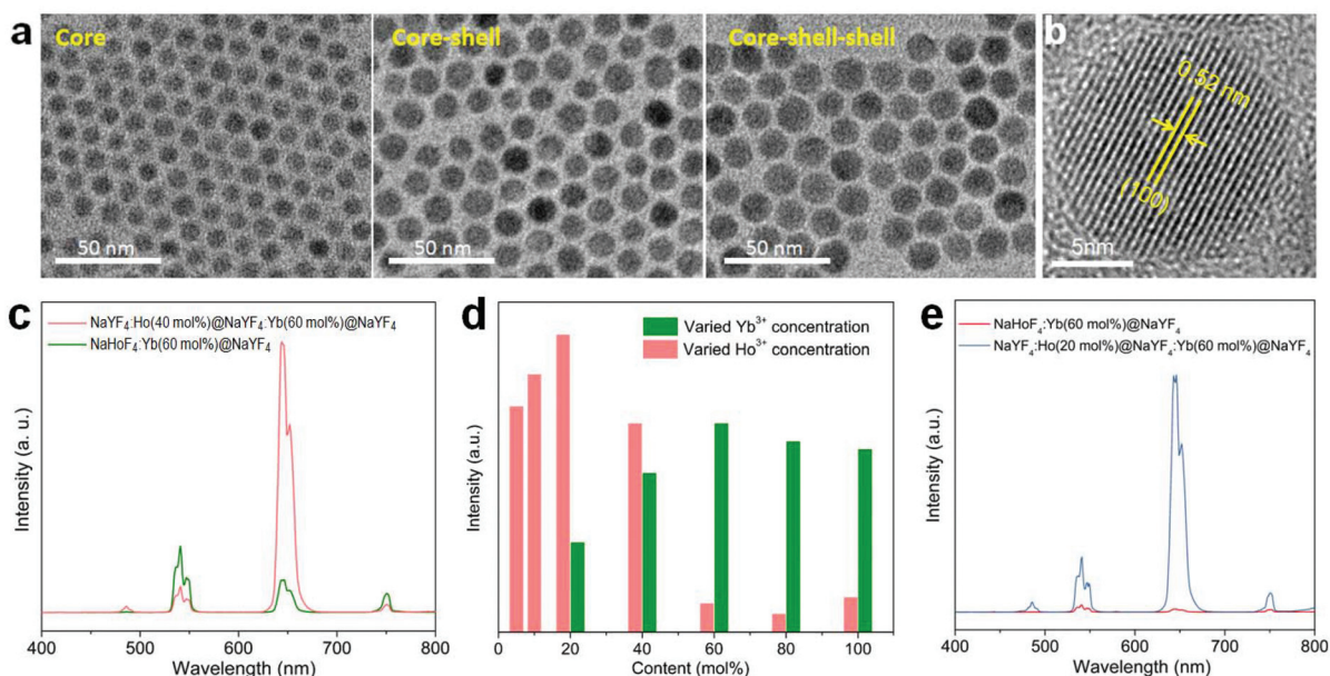
Fig. 3 (a) TEM images of the \text{NaF}_4\text{:Ho(40 mol\%)}@ \text{NaF}_4\text{:Yb(60 mol\%)}@ \text{NaF}_4 core-shell-shell nanoparticles. (b) The high-resolution TEM image of the core-shell-shell nanoparticles. (c) A comparison of the upconversion emission spectra of as-prepared \text{NaF}_4\text{:Ho(40 mol\%)}@ \text{NaF}_4\text{:Yb(60 mol\%)}@ \text{NaF}_4 core-shell-shell and \text{NaHoF}_4\text{:Yb(60 mol\%)}@ \text{NaF}_4 core-shell nanoparticles under 980 nm excitation. (d) Dependence of the overall upconversion emission intensity of the \text{NaF}_4\text{:Ho(5–100 mol\%)}@ \text{NaF}_4\text{:Yb(20–100 mol\%)}@ \text{NaF}_4 core-shell-shell nanoparticles with a tuning of the concentrations of \text{Ho}^{3+} in the core and \text{Yb}^{3+} in the interlayer, respectively. (e) Comparative upconversion emission spectra from the optimized \text{NaF}_4\text{:Ho(20 mol\%)}@ \text{NaF}_4\text{:Yb(60 mol\%)}@ \text{NaF}_4 core-shell-shell nanoparticles and \text{NaHoF}_4\text{:Yb(60 mol\%)}@ \text{NaF}_4 core-shell nanoparticles under identical measurement conditions.
