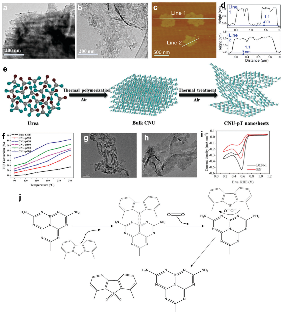
Fig. 18 TEM images of C 3 N 4 nanomesh at synthesis temperatures of (a) 500 °C and (b) 600 °C and (c) an AFM image of C 3 N 4 nanomesh at 600 °C with (d) the height profile of lines in the AFM image. Reprinted with permission. 210 Copyright 2018, Royal Society of Chemistry. (e) Synthesis route of C 3 N 4 nanosheets from urea. (f) Conversion of hydrogen sulfide with the help of O 2 by bulk g-C 3 N 4 and g-C 3 N 4 nanosheets formed at different oxidation temperatures of 350 °C, 450 °C, 500 °C, 550 °C and 600 °C. Reprinted with permission. 211 Copyright 2019, American Chemical Society. TEM images of (g) B-C 3 N 4 and (h) g-C 3 N 4 . Reprinted with permission. 212 Copyright 2019, Elsevier B.V. (i) Cyclic voltammety curves for B-C 3 N 4 and BN. Reprinted with permission. 213 Copyright 2020, Elsevier Inc. (j) Oxidation mechanism of 4,6-DMDBT with O 2 molecules by B-C 3 N 4 . Redrawn with permission. 212 Copyright 2019, Elsevier B.V.
