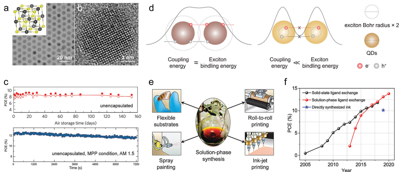
Fig. 1 (a) Typical transmission electron microscopy (TEM) images of PbS QCDs. The inset shows the crystal structure of PbX. (b) High-resolution TEM image of a single PbS QD. Reprinted with permission from ref. 23. Copyright 2014, American Chemical Society. (c) The air-stability (top) and photo-stability (bottom) of PbS QCD solar cells in air ambient. Reprinted with permission from ref. 8. Copyright 2014, Nature Publishing Group (top). Reprinted with permission from ref. 24. Copyright 2019, Nature Publishing Group (bottom). (d) Schematic description of the effect of quantum confinement effect on exciton dissociation in coupled QCD assemblies. For QDs with strong quantum confinement effect/large exciton Bohr radius (e.g. PbX), the inter-NC coupling energy between the QDs is comparable with their exciton binding energy, which enables the excitons to dissociate without the aid of an external potential gradient. Whereas, the exciton recombination is preferable for the QDs that assemble with a small exciton Bohr radius (e.g. CdX). (e) The solution-phase synthesis of PbX QCDs is compatible with all industrial deposition techniques. Reprinted with permission from ref. 25 Copyright 2012, Nature Publishing Group. (f) Efficiency progress of PbS QCD solar cells.
