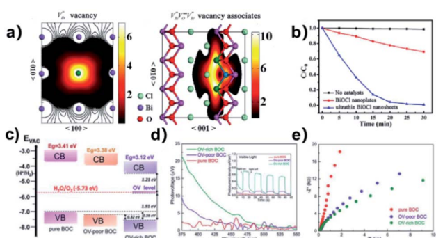
Fig. 13 Schematic representation of the trapped positrons of (a) V_{\text{Bi}} defect and V_{\text{Bi}} V_{\text{O}} V_{\text{Bi}} vacancy associates, respectively. (b) Comparison of the photodecomposition of Rhodamine B with ultrathin BiOCl nanosheets and BiOCl nanoplates under simulated solar irradiation. (c) Schematic illustration of the band structure of O V -rich/poor BOC and pure BOC. (d) Surface photovoltage spectrum of O V -rich/poor BOC and pure BOC. Current density transients of O V -rich/poor BOC and pure BOC under visible-light irradiation are shown in the inset. (e) Nyquist impedance plots of O V -rich/poor BOC and pure BOC. Reproduced with permission from ref. 142 Copyright 2013, the American Chemical Society, and ref. 143 Copyright 2018, The Royal Society of Chemistry.
