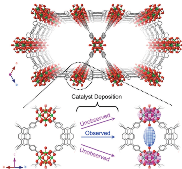
Fig. 15 Assembly of NU-1000 with stress on observed electron density of metal ions after post-synthetic anchoring of metal sites [reprinted with permission from ref. 154, Copyright © American Chemical Society, 2018].
