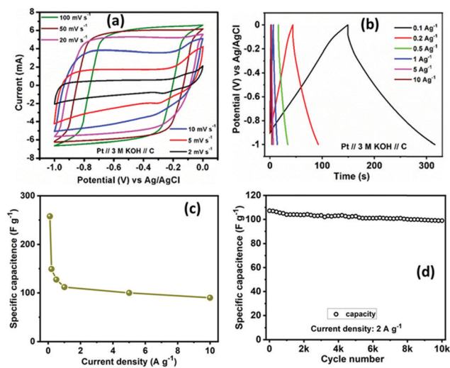
Fig. 7 Electrochemical supercapacitor performances of the PSCN electrode in a three-electrode configuration. (a) cyclic voltammograms at various scan rates at 0.0 to -1.0 V, (b) GCD profile at 0.1 to 10 \text{A g}^{-1} current density, (c) variation of specific capacitance vs. current density, and (d) cycling stability test at 2 \text{A g}^{-1} current density for 10\,000 cycles.
