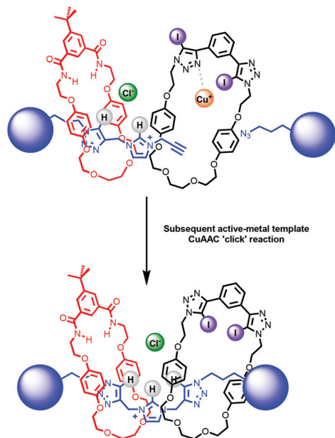
Fig. 5 Schematic representation of route to hetero[3]rotaxane combining chloride anion-templated and active-metal templated methodologies.
