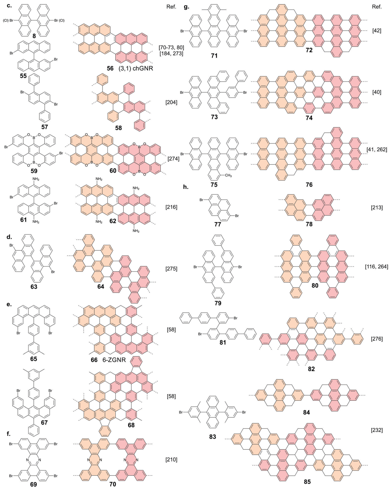
Fig. 3 Register of precursors used so far for atomically precise GNR formation together with the resulting GNR structure. (a) Armchair GNRs, excluding ones resulting from the lateral fusion of ribbons. (b) Chevron-like GNRs. (c) Chiral GNRs. (d) Cove-edged GNRs. (e) zigzag GNRs. (f) Porous GNR. (g) GNRs with embedded topological states. (h) GNRs with other edge topology.
