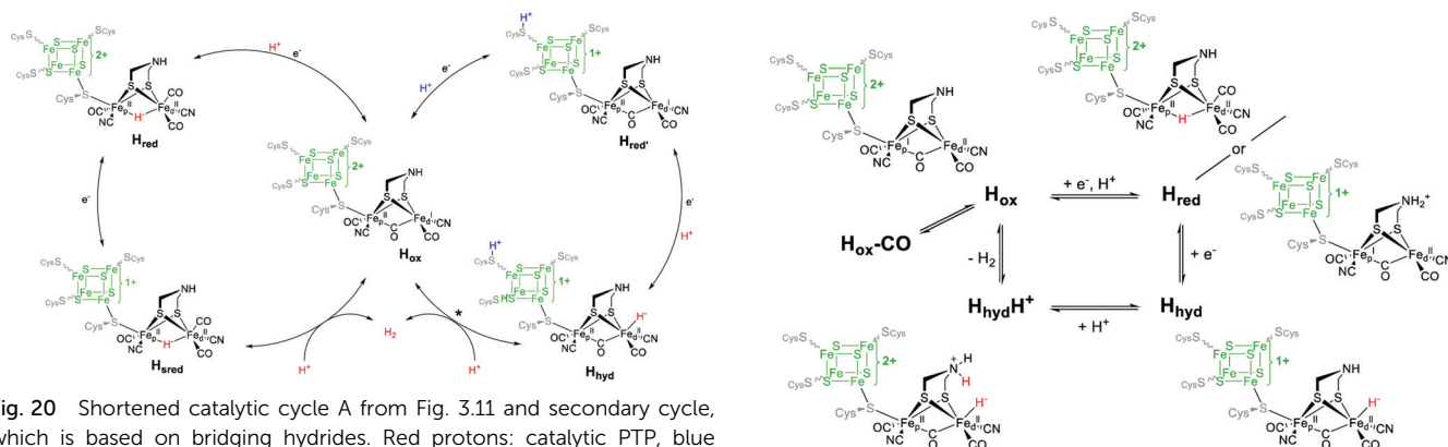
Fig. 21 Schematic representation of the catalytic cycle of [FeFe]-hydrogenase, based on the states observed under whole-cell conditions including the protonated hydride species ( H_{hyd}H^+ ). Figure and caption from ref. 35.
