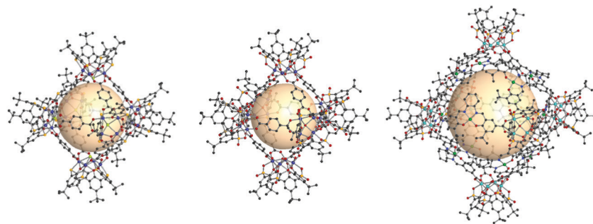
Fig. 13 Structural illustration of [\text{Co}_4\text{Cl}(\text{BTC4A})]_6(\mathbf{A1})_{12} (left), 68 [\text{Co}_4\text{O}(\text{TBSC})]_6(\mathbf{A1})_{12} (middle), 69 and [\text{Zn}_4\text{O}(\text{TBSC})]_6(\mathbf{A1})_{12} (right). 14
