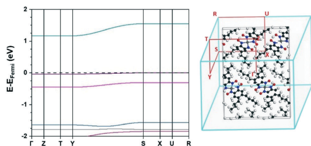
Fig. 4 Electronic band structure (left) and Brillouin zone k -point path (right) of the ambient pressure structure of [Pt(bqd-dibutyl) 2 ]. E Fermi = -4.99 eV.
