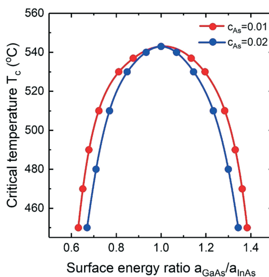
Fig. 7 Critical temperature versus the ratio of binary surface energy terms for InGaAs materials system at fixed As concentration of c_{\text{As}} = 0.01 (red curve) and c_{\text{As}} = 0.02 (blue curve). The dots represent numerical calculations and the solid curves are polynomial fits.
