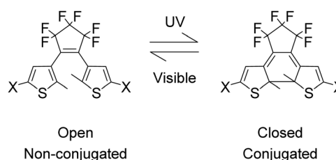
Fig. 1 Photochromism of dithienylethene (DTE) derivatives.
