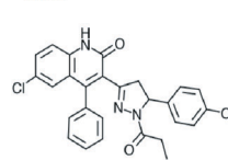
Fig. 5 Inhibitors of DSB repair by (A) NHEJ and (B) HR.
