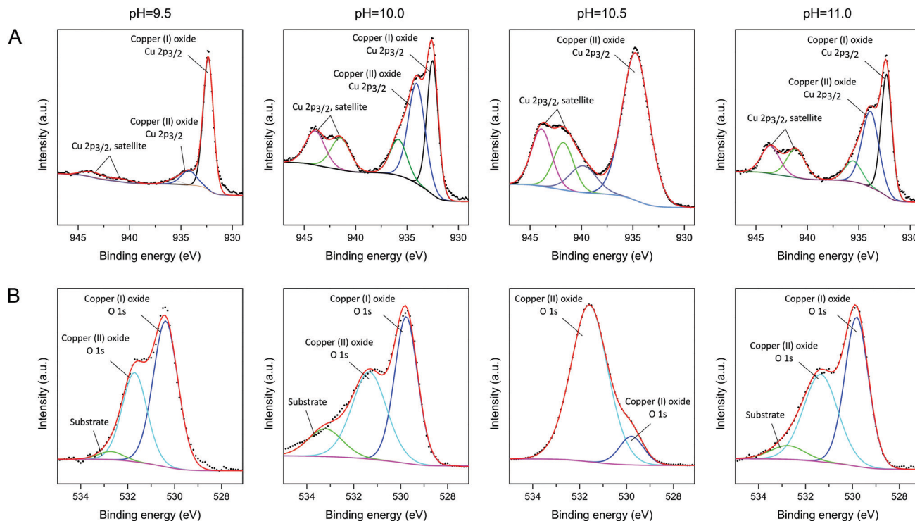
Fig. 3 High-resolution XPS patterns of the Cu x O samples produced at different pH. (A) Deconvoluted XPS patterns of the Cu 2p 3/2 region and (B) O 1s region.
