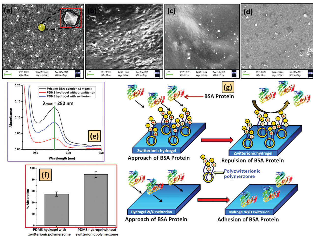
Fig. 6 FESEM images of (a) BSA protein cast over the glass slide; (b) BSA protein adsorbed over the PDMS based hydrogel without (w/o) entrapped polyzwitterionic polymerzomes; BSA protein adsorbed over the PDMS based hydrogel having entrapped polyzwitterionic polymerzomes at (c) the initial day of study and (d) after 7 days of dipping into BSA solution; (e) analysis of the BSA adsorption through UV-vis analysis; (f) protein adsorption (%) over the hydrogel surface calculated using the calibration curve and (g) schematic of the antifouling activity of the hydrogel.
