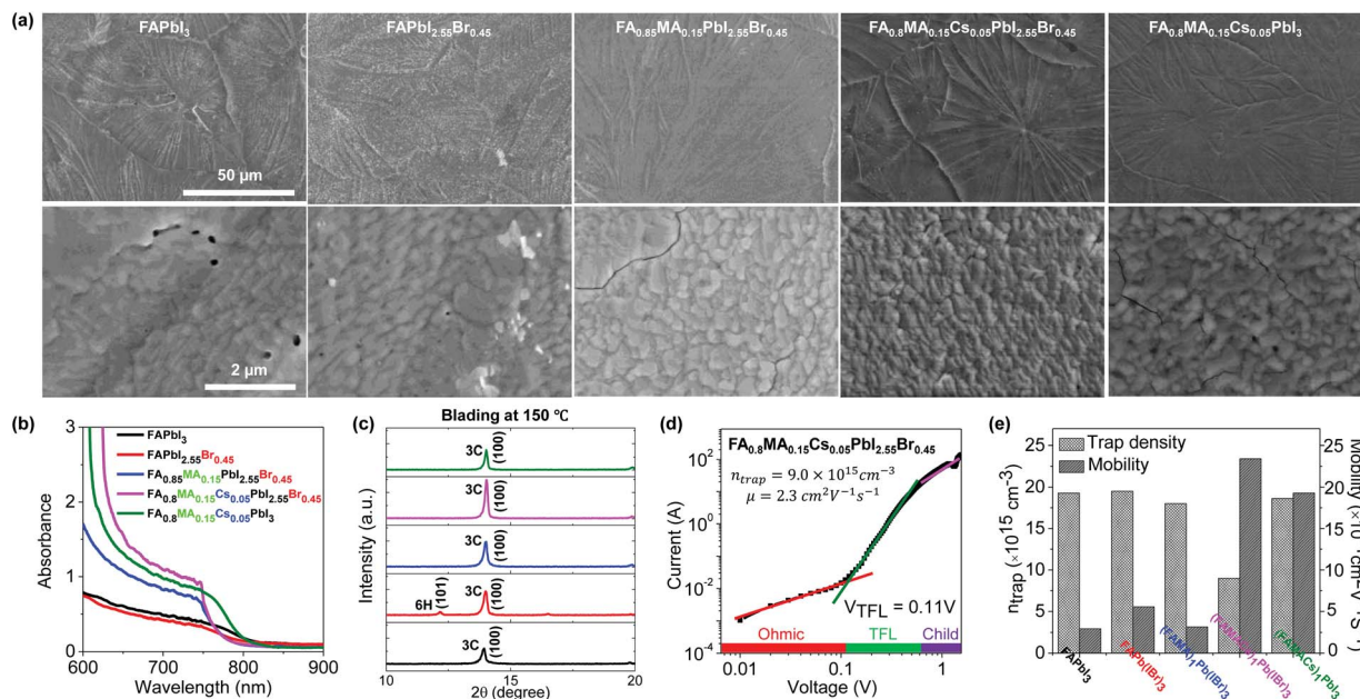
Fig. 3 Comparison of FAPbl 3 , FAPbl 2.55 Br 0.45 , FA 0.85 MA 0.15 Pbl 2.55 Br 0.45 , FA 0.8 MA 0.15 Cs 0.05 Pbl 3 and FA 0.8 MA 0.15 Cs 0.05 Pbl 2.55 Br 0.45 films via blade coating. (a) Top-view SEM images of perovskite films prepared using the blade coating method at 150 °C (top row shows low magnification while the bottom row shows higher magnification images). (b and c) Absorption spectra and XRD patterns of blade coated hybrid perovskite as-cast thin films with different precursor inks. (d) Dark I - V measurement of the electron-only device displaying V_{TFL} kink point behavior for the representative FA 0.8 MA 0.15 Cs 0.05 Pbl 2.55 Br 0.45 perovskite thin film. (e) Trap density and electron mobility.
