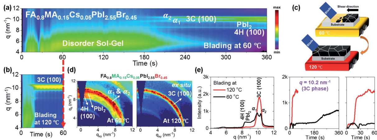
Fig. 2 In situ 2D GIWAXS intensity map of the FA 0.8 MA 0.15 Cs 0.05 Pbl 2.55 Br 0.45 perovskite precursor inks showing ink-to-solid transformation during blade coating (a) at 60 °C and (b) 120 °C. (c) Schematic representation of the FA 0.8 MA 0.15 Cs 0.05 Pbl 2.55 Br 0.45 perovskite thin film formation mechanism at low 60 °C and high 120 °C blade coating temperatures. (d) Representative 2D GIWAXS snapshots taken at the final stage of blade coating perovskite films for FA 0.8 MA 0.15 Cs 0.05 Pbl 2.55 Br 0.45 at 60 °C and 120 °C, respectively. (e) Scattering vector q versus intensity distribution of the FA 0.8 MA 0.15 Cs 0.05 Pbl 2.55 Br 0.45 perovskite film at the final stage of blade coating and time evolution of the diffraction intensity related to the perovskite 3C (100) phase ( q = 10.2 nm -1 ) for FA 0.8 MA 0.15 Cs 0.05 Pbl 2.55 Br 0.45 perovskite ink at 60 °C and 120 °C.
