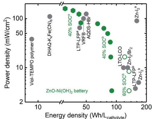
Fig. 6 Ragone plot of static semi-solid battery (Zn– \text{Ni}(\text{OH})_2 ) and reported redox flow battery chemistry including Viol–TEMPO polymer, 63 DHAQ– \text{K}_4\text{Fe}(\text{CN})_6 , 14 AQDS–HBr, 9 LTO–LCO, 26 LTP–LFP a , 4 LTP–LFP b , 62 VRFB, 12 Zn– \text{I}_2/\text{Br}_2 , 35 Zn– \text{I}_2^a , 38 and Zn– \text{I}_2^b . 61 The Zn–Ni semi-solid battery chemistry shown from this work contains anolyte with 5.2 vol% ZnO and catholyte with 7.6 (green hexagon, 40% SOC a ) and 12.5 vol% \text{Ni}(\text{OH})_2 (green solid 40% SOC b and open circles 60% SOC b ). Abbreviations: AQDS: 9,10-anthraquinone-2,7-disulphonic acid, DHAQ: 2,6-dihydroxyanthraquinone, TEMPO: 2,2,6,6-tetramethylpiperidinyloxy, Viol: viologen, LTP: \text{LiTi}_2(\text{PO}_4)_3 , LFP: \text{LiFePO}_4 , LTO: \text{Li}_4\text{Ti}_5\text{O}_{12} .
