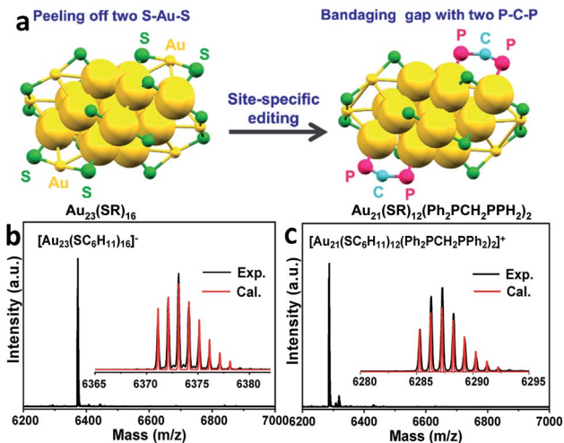
Fig. 3 (a) A schematic diagram of the site-specific editing of \text{Au}_{23}(\text{SR})_{16} by resecting two \text{RS-Au-SR} motifs and bandaging the gaps with two \text{Ph}_2\text{P-CH}_2\text{-PPh}_2 staples to obtain \text{Au}_{21}(\text{SR})_{12}(\text{Ph}_2\text{PCH}_2\text{PPh}_2)_2 . Color codes: yellow = Au; green = S; pink = P; blue = C. Carbon tails are omitted for clarity. SR = cyclohexanethiol. The ESI-MS spectra of (b) [\text{Au}_{23}(\text{SC}_6\text{H}_{11})_{16}]^- and (c) [\text{Au}_{21}(\text{SC}_6\text{H}_{11})_{12}(\text{Ph}_2\text{PCH}_2\text{PPh}_2)_2]^+ .
