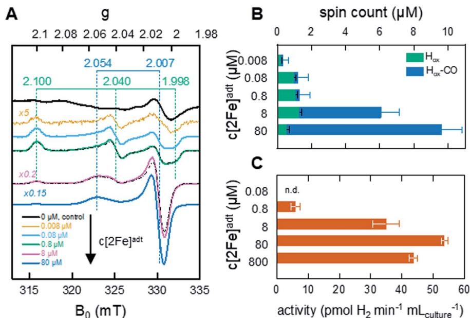
Fig. 2 In vivo H-cluster assembly monitored by EPR spectroscopy and \text{H}_2 gas production. (A) Whole-cell EPR spectra of apo-HydA1 (control, 0 \mu\text{M} [2\text{Fe}]^{\text{adt}} added) and [2\text{Fe}]^{\text{adt}} -HydA1 containing cell suspensions, concentrated to 400 \mu\text{L} . H-cluster assembly occurs spontaneously upon addition of [2\text{Fe}]^{\text{adt}} to the medium, with \text{H}_{\text{ox}} being the favored state at low [2\text{Fe}]^{\text{adt}} concentrations. As the concentration of the synthetic cofactor increases, the cell samples become dominated by the \text{H}_{\text{ox}}\text{-CO} state. The g -values of \text{H}_{\text{ox}} (green dashed lines) and \text{H}_{\text{ox}}\text{-CO} (blue dashed lines) states are based on simulations of the two samples at 0.8 and 8 \mu\text{M} (black dash-dotted lines). All [2\text{Fe}]^{\text{adt}} -HydA1 spectra were corrected for contribution from the cells by subtracting the signal of the apo-HydA1 control sample (black spectrum). EPR experimental conditions: T = 20 \text{ K} , P = 1 \text{ mW} , \nu = 9.28 \text{ GHz} . (B) Concentrations of the \text{H}_{\text{ox}} (green bars) and \text{H}_{\text{ox}}\text{-CO} (blue bars) signals in each sample, extrapolated from the simulations. The full length of the bar reflects total spin count. Error bars indicate estimated relative error from simulations, in addition an absolute error of approx. 0.5 \mu\text{M} is expected from the background subtraction (see Fig. S1† for details). (C) Average rate of hydrogen gas production during 1 h from anaerobic 2 mL E. coli cultures, concentrated from 100 mL batch cultures.
