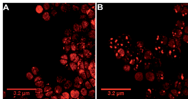
Fig. 4 Super-resolution SIM imaging revealing localization of 4 4+ in S. aureus SH1000 cells at (A) 5 min and (B) 60 min. Cells images using the emission of 4 4+ on excitation at 450 nm using the A568 filter. After treatment with 4 μM 4 4+ , cells were washed with PBS before fixing with paraformaldehyde (4%).
