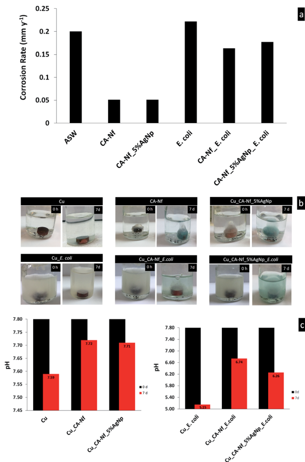
Fig. 7 Cu, Cu coated CA-Nf and Cu coated CA-Nf with 5% AgNps in the ASW and ASW inoculated with E. coli for 7 days. Also, Fig. 7 shows photographs of the Cu discs weight loss analysis in ASW and ASW inoculated with bacterium. It obviously shows that the corrosion rates decrease with the presence of CA-Nf coatings in both ASW and ASW inoculated with bacterium. The observed decreased corrosion rates are associated with larger surface
